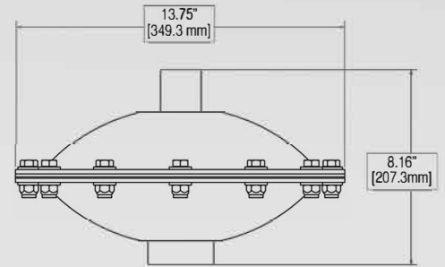
For 1.5" & 2" Pumps
