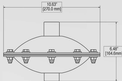
For 1" Pumps
